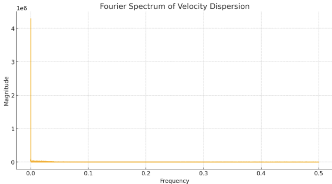
Figure 3.7-A (Fourier spectrum of velocity dispersion, SDSS DR8): Low-frequency dominance consistent with long-wavelength chirality waves driving cosmic acceleration.
