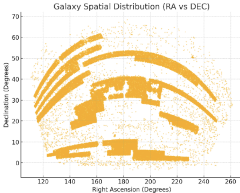
Figure 3.5-A (SDSS DR8 RA–DEC density map): Raw galaxy clustering used as input to CWT analysis.
