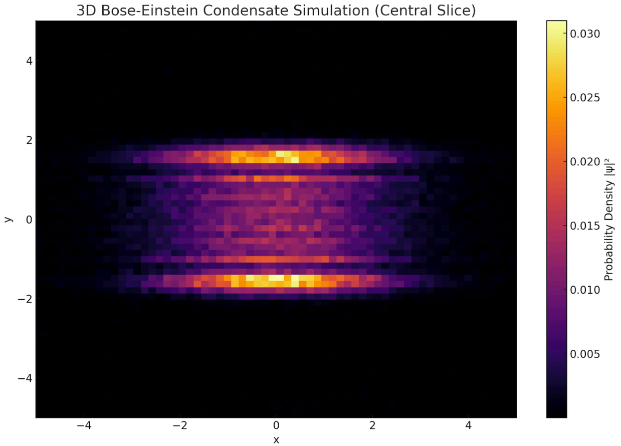
Figure C. 3D Bose-Einstein Condensate Simulation (Central Slice) — Central slice illustrates chirality-driven vortex formation, where phase-locked asymmetry induces structured coherence in the condensate.
