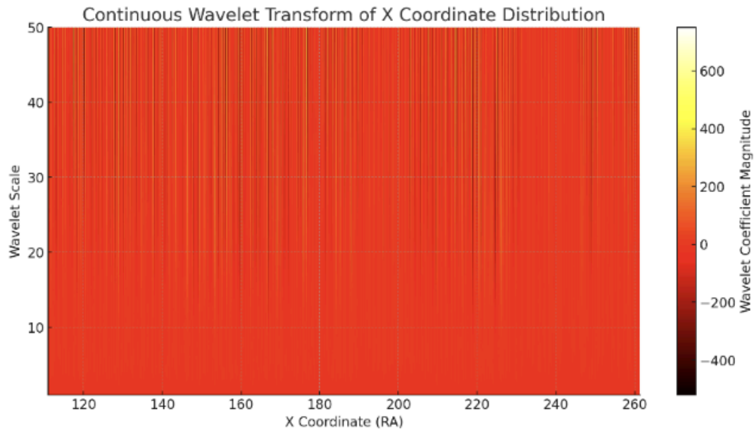
Figure 3.5-D (CWT coefficient map, SDSS DR8): Raw wavelet coefficients (RA \times scale), showing the resonance coefficient field.
