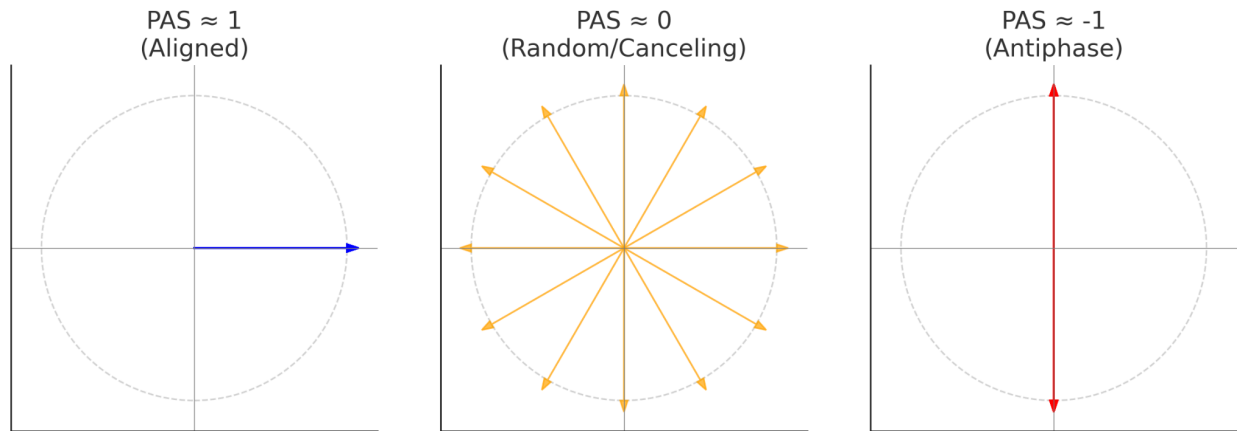
Diagram: Circle plots with vectors showing PAS \approx 1 (aligned), PAS \approx 0 (random/canceling), PAS \approx -1 (antiphase).
