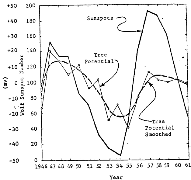
Figure 3. Yearly average tree potentials and sunspot numbers.
