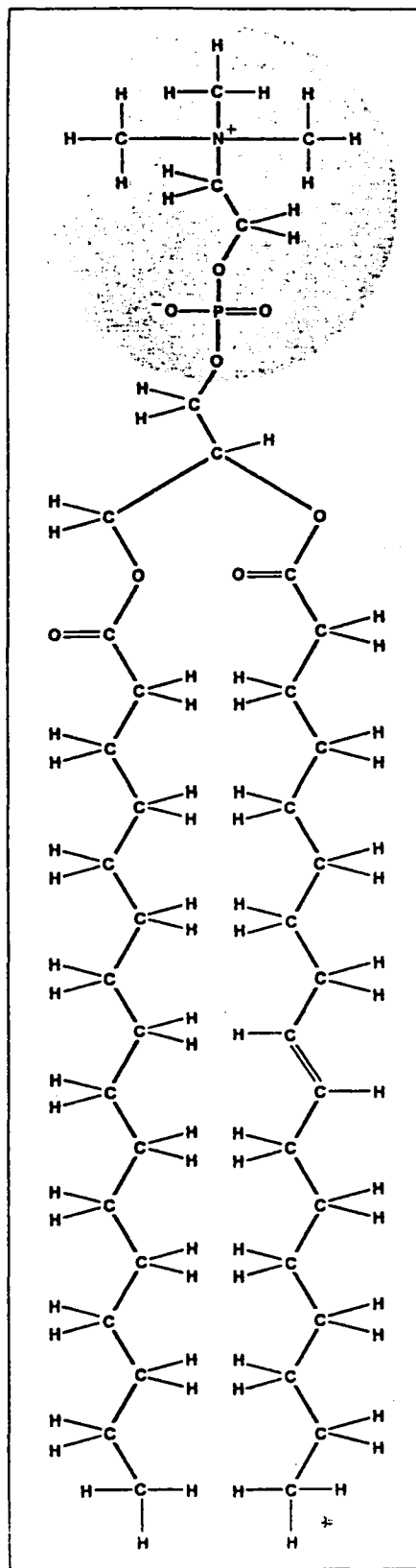
FIG. 38. CHEMICAL COMPOSITION OF A LIPID MOLECULE (FROM CAPALDI, 1976).
