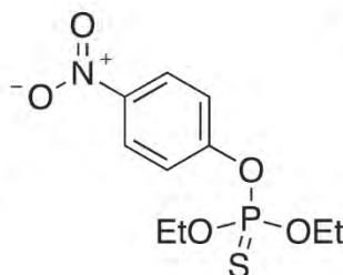
Parathion synthetic
