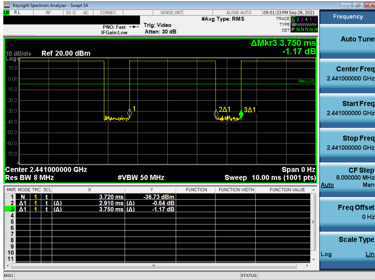
Bluetooth Antenna 2 Transmission Plot
