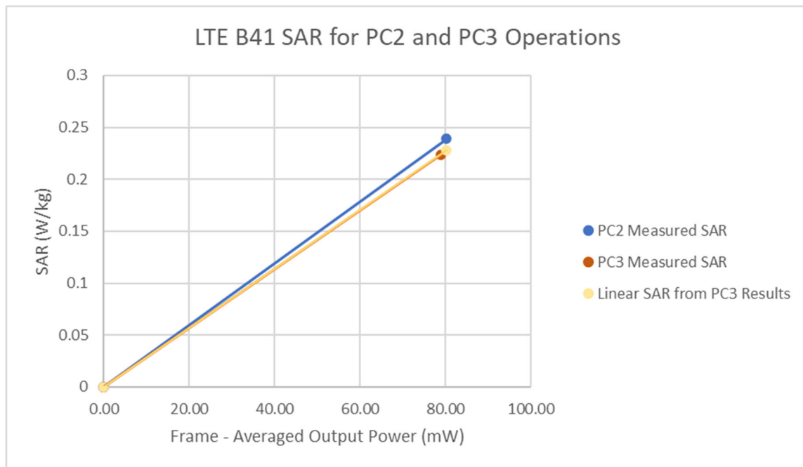
Figure 13-5 LTE Band 41 Hotspot Linearity
